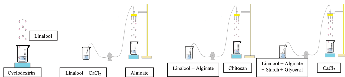
Figure 1. Schematic diagrams of the experimental setup corresponding to (a) chemical precipitation, (b) inverse gelation, (c) coacervation, and (d) oil-entrapped-emulsion.
